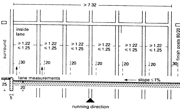
⑧ Dimensions: running track type B
